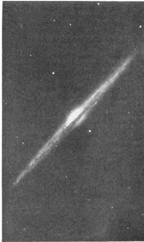
THE NEBULA SEEN EDGE-ON
