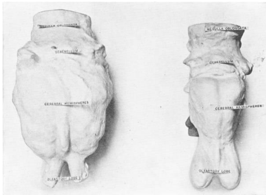
COMPARATIVE SIZES OF BRAINS OF RHINOCEROS AND DINOCERAS Nat. Hist. Mus.
